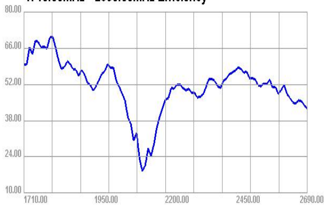
1710.00MHz - 2690.00MHz Efficiency
