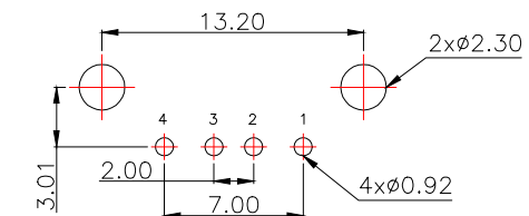
PCB.WELDING DRAWING (TOLERANCE:±0.05)
